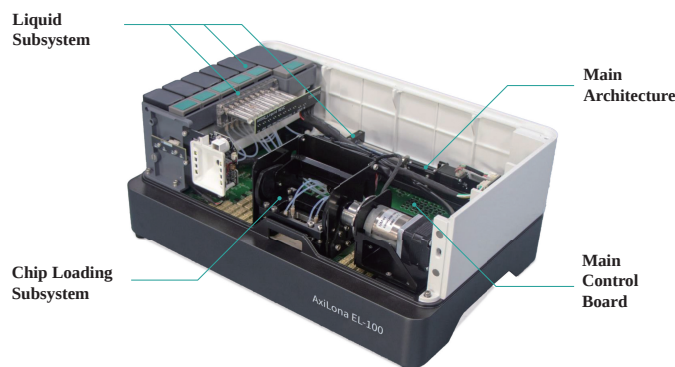
Key Components of AxiLona EL-100
