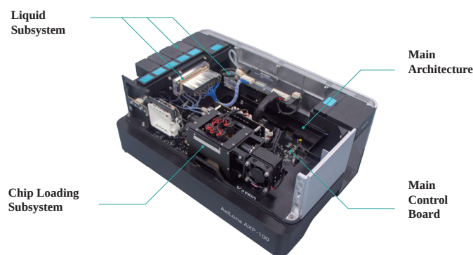
Key Components of AxiLona AXP-100
