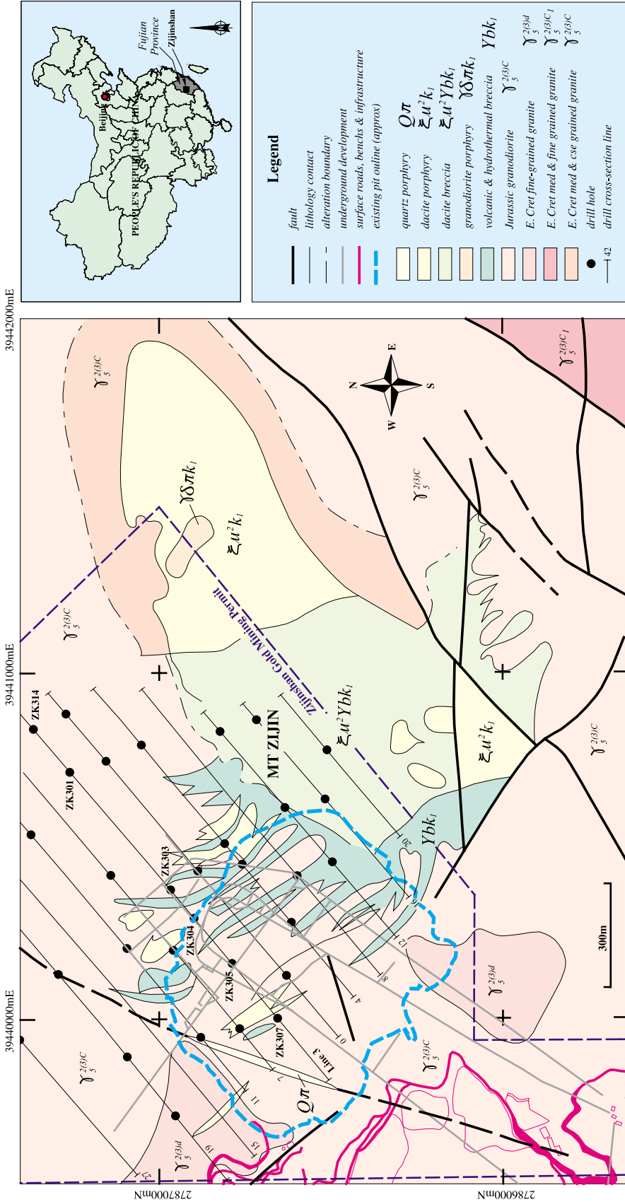
Figure 4.1 Zijinshan - Location and Project Area Geology
