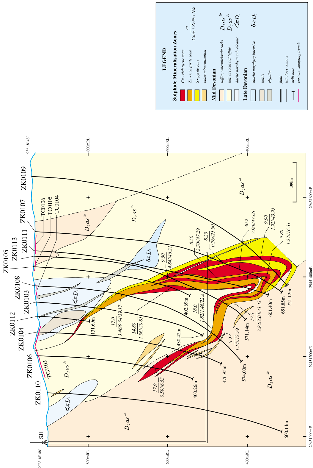
Figure 4.11 Ashele - Cross Section Line 1
