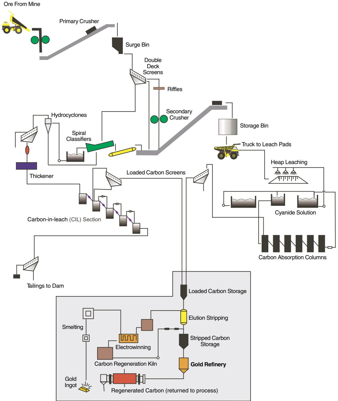
Figure 8.1 Zijinshan - Metallurgical flow chart for the Gold Mine
