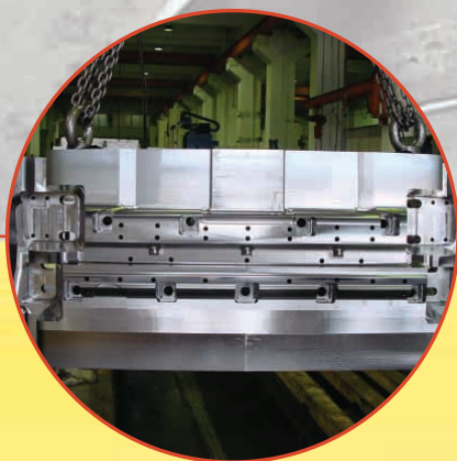
Motor vehicle bumper mould base 汽車用保險桿模架
