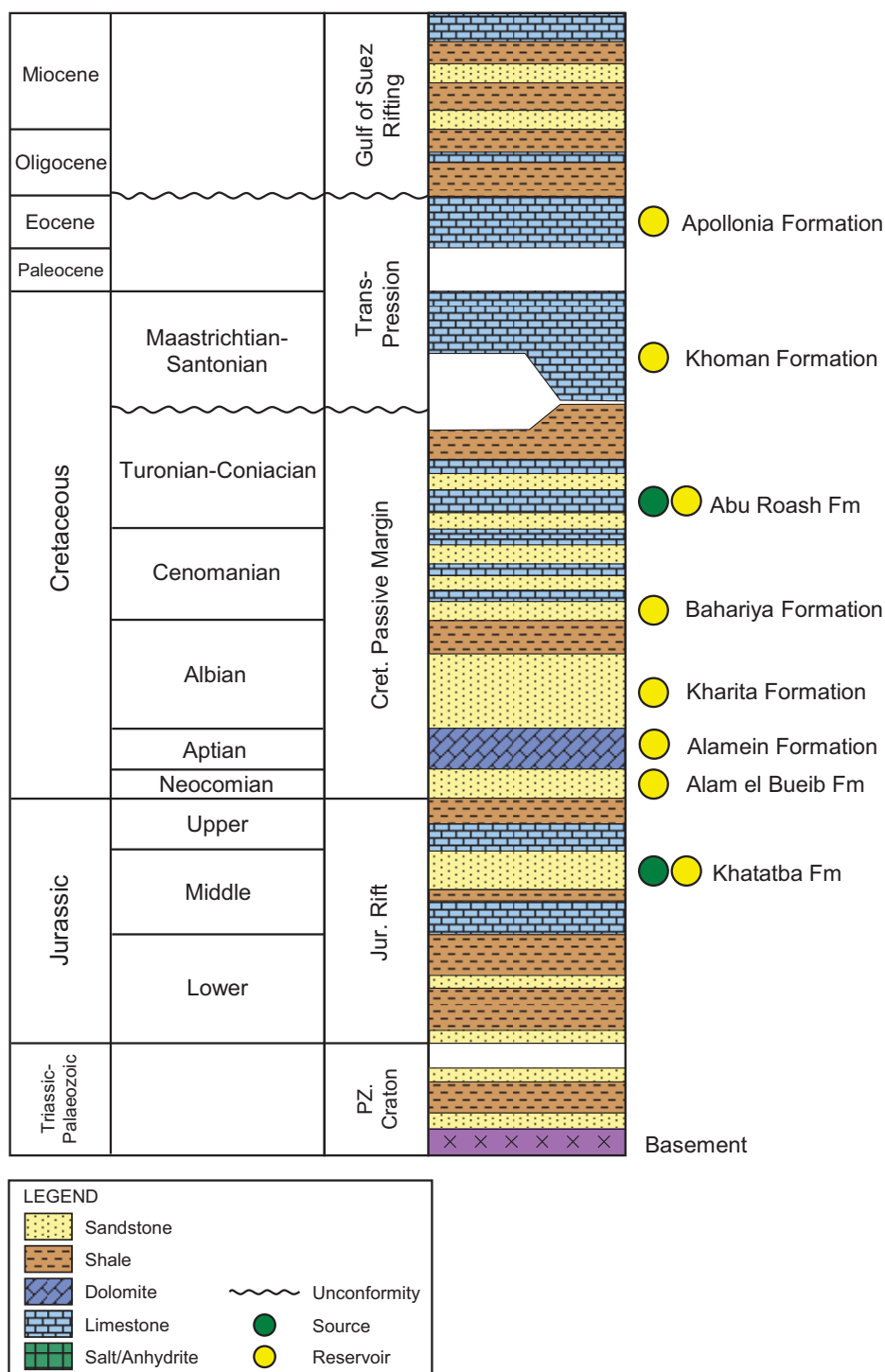
Figure 22: Composite Stratigraphy, Abu Sennan and BEA, Egypt
