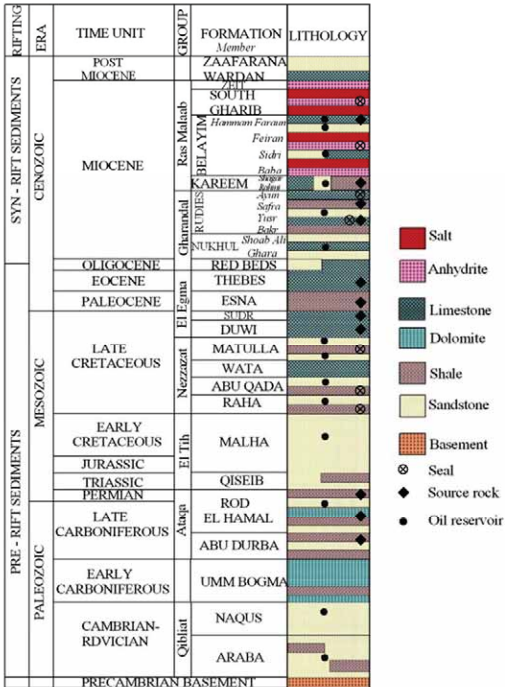
Figure 15: Generalised Stratigraphy, Eastern Desert, Egypt
