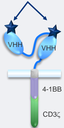
Cilta-cel (CAR-T)
