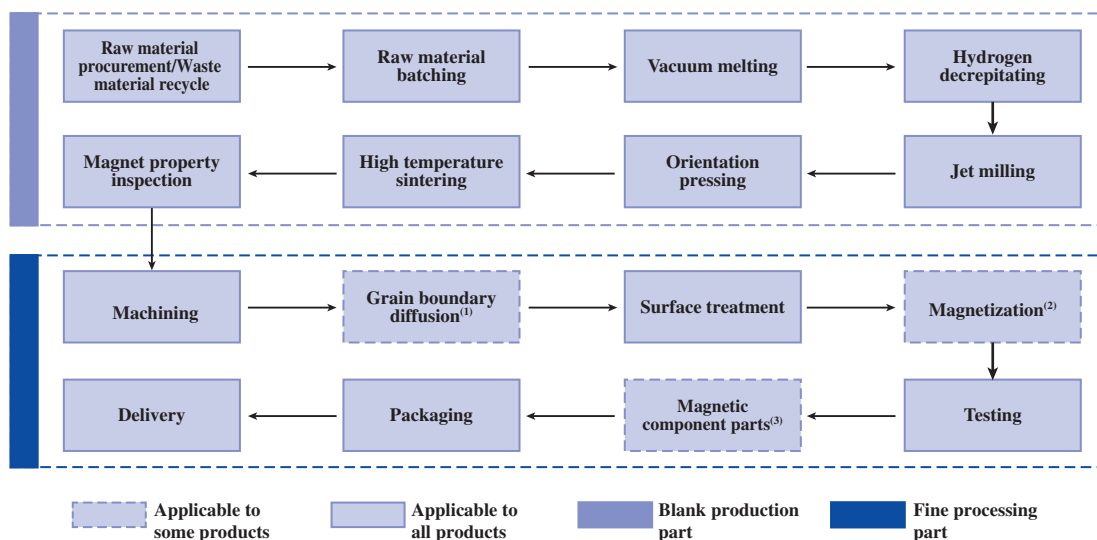
Production Workflow
