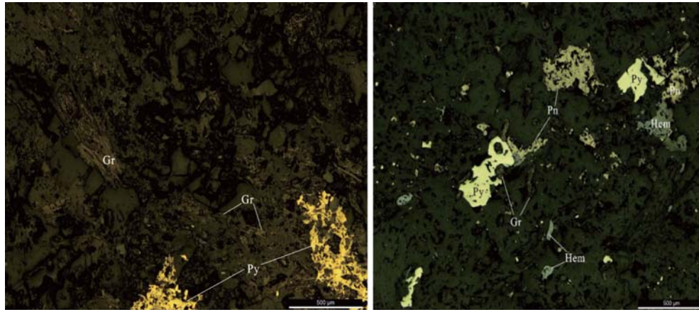
Figure 4–5: Petrographical analysis
