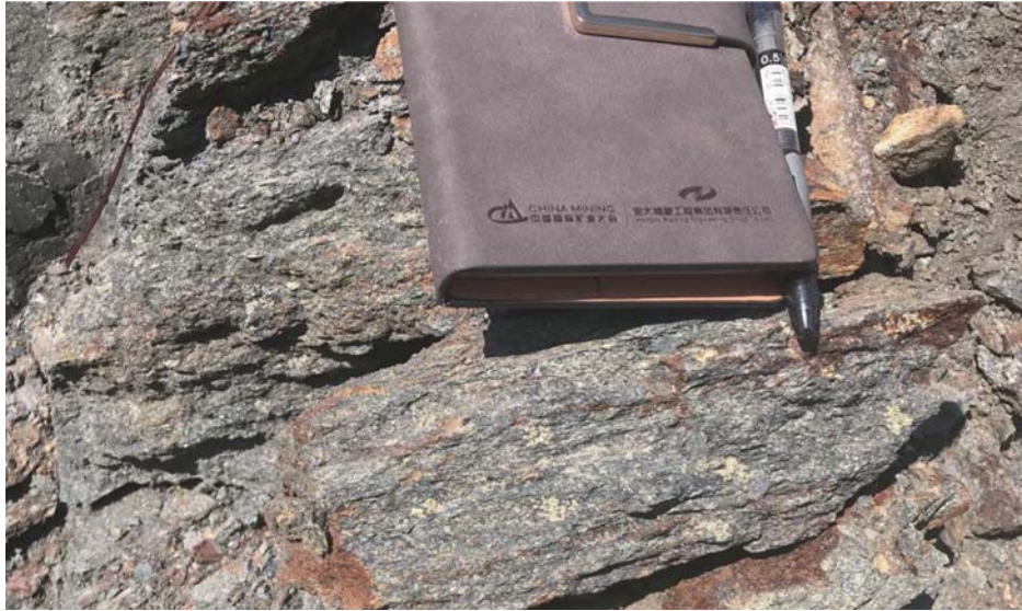
Figure 4–3: Graphitic schist
