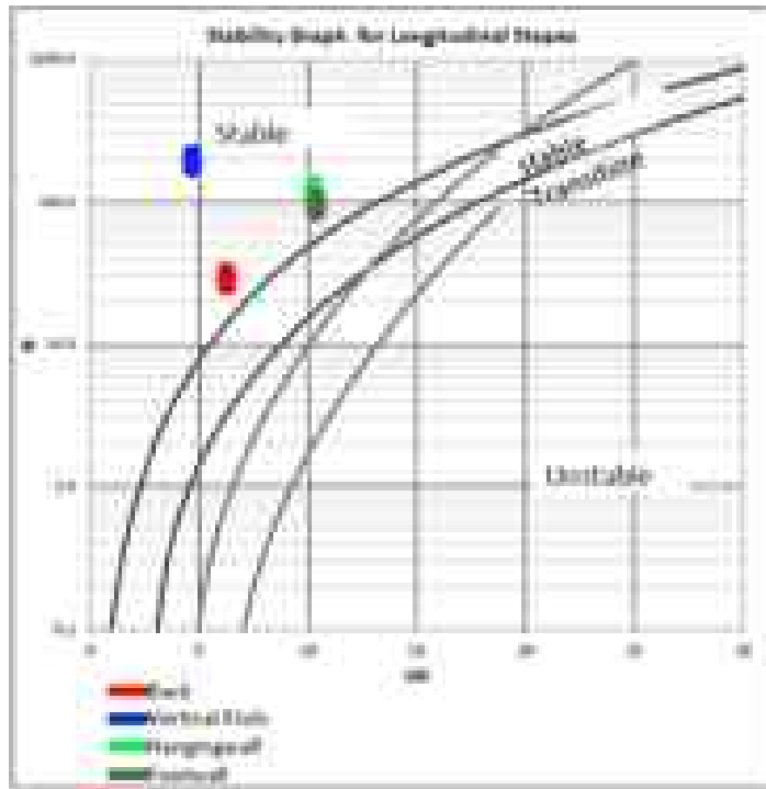
Figure 12-8: Mathews Stability Graph, Longitudinal Stopes (Mathews et al, 1981)
