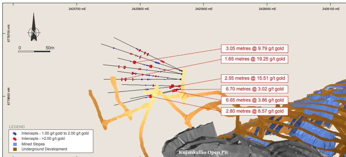
Figure 7 – Basin Zones-1 Plan View.
