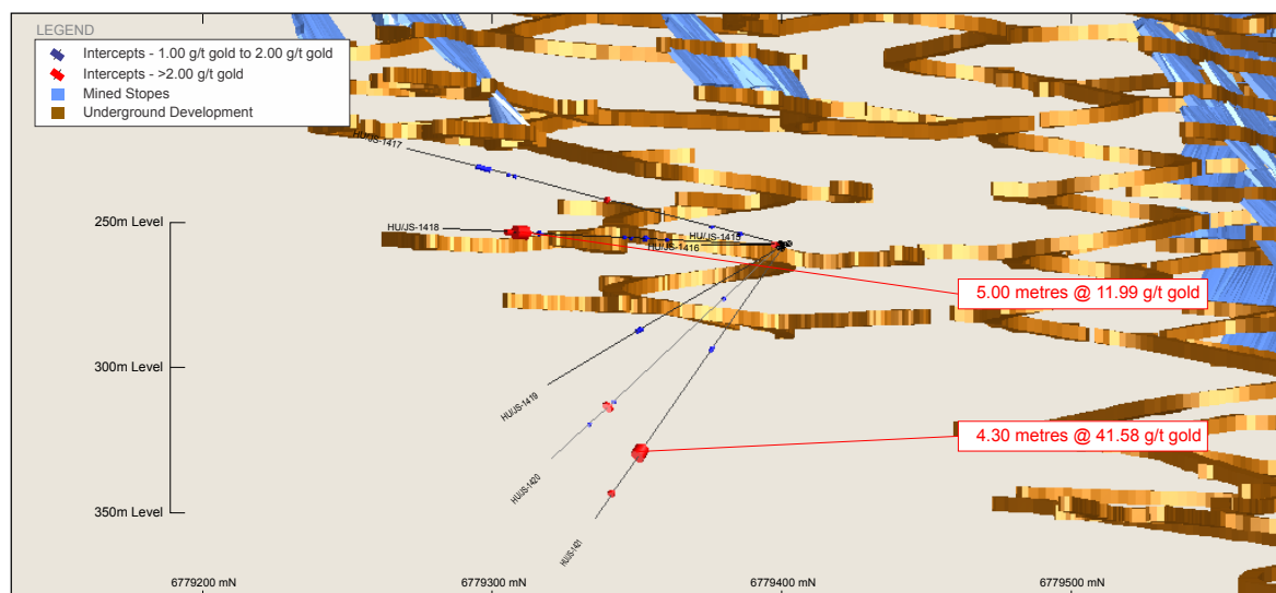
Figure 6 – Arpola-2 Vertical Section. View looking west.
