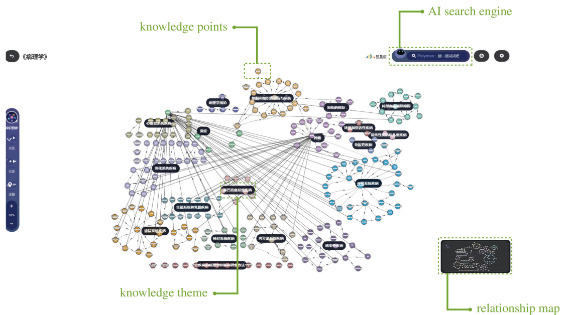
Knowledge Graph
