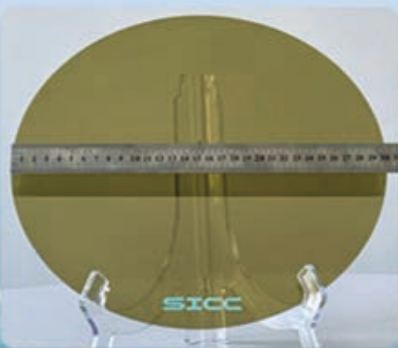
12-inch conductive n-type silicon carbide substrate
