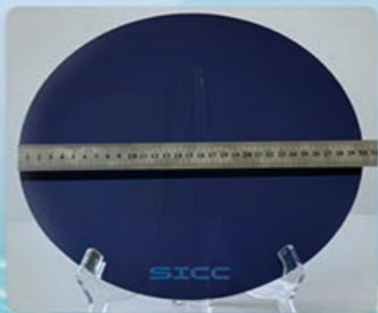
12-inch conductive p-type silicon carbide substrate
