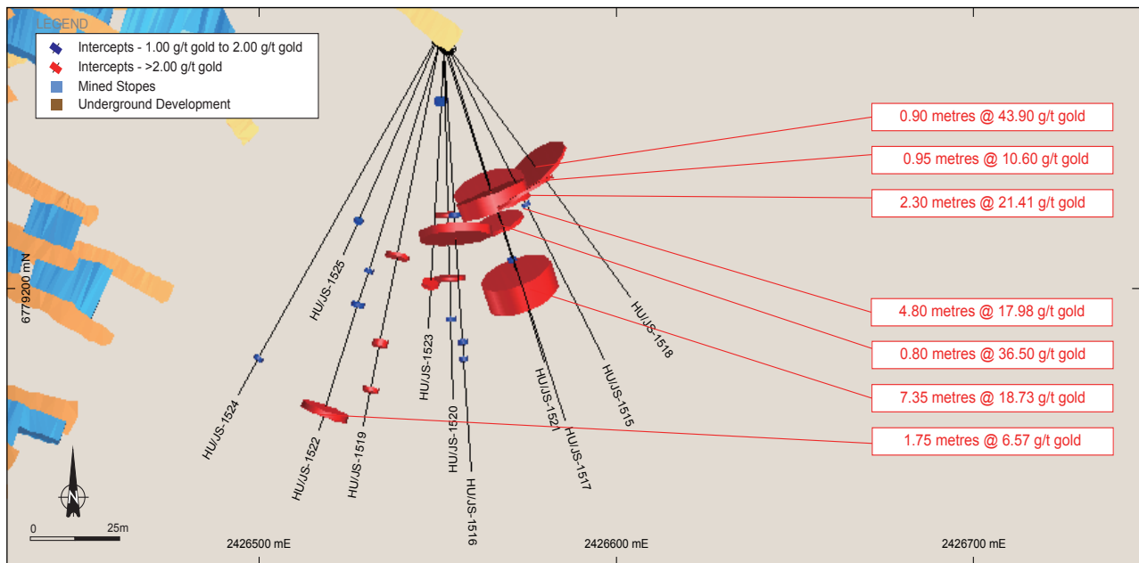
Figure 5 – Plan view of the 2025 Arpola-7 campaign highlighting intercepts \geq 10 gram*metres.
