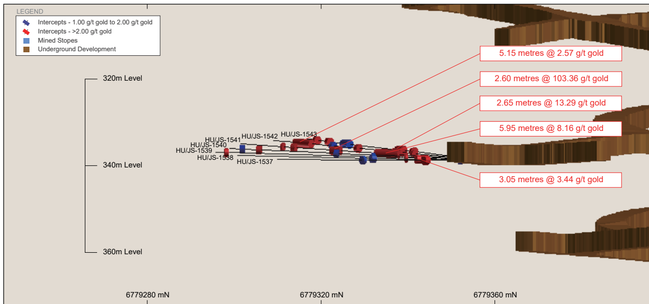
Figure 7 – Plan view of the 2026 Arpola-2 campaign highlighting intercepts \geq 10 gram*metres.
