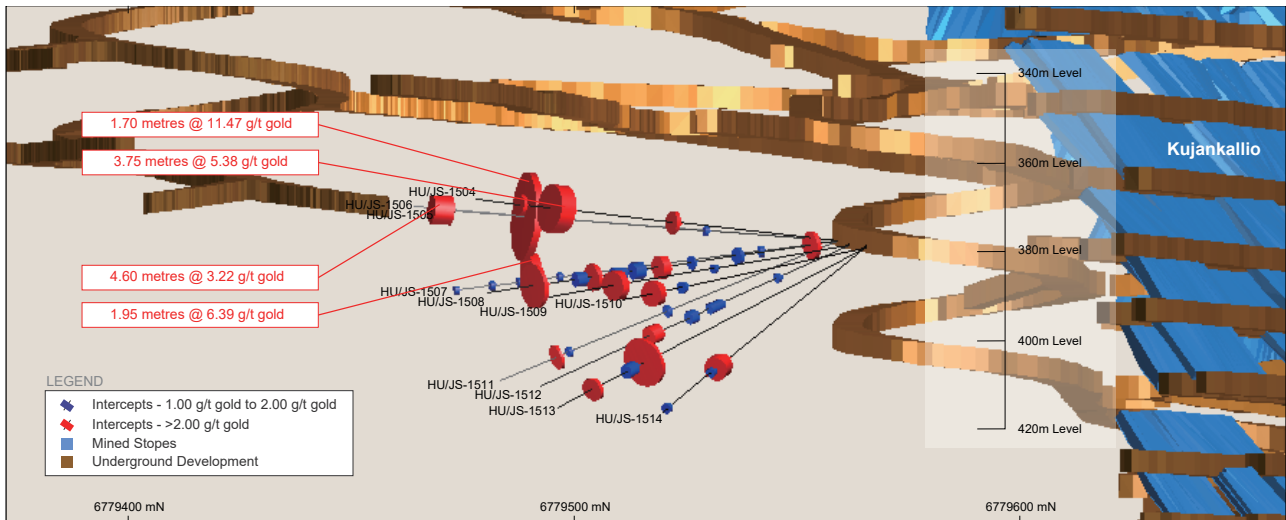
Figure 4 – Vertical view of the Arpola-6 campaign highlighting intercepts \geq 10 gram*metres. View looking east.
