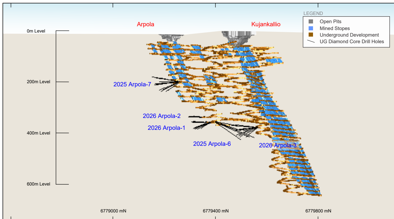
Figure 3 – Jokisivu Gold Mine displaying reported drilling campaigns. View looking west.
